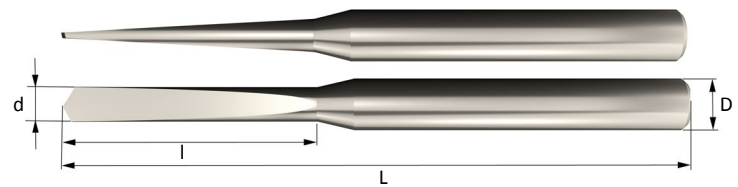
Style F | Carbide Spade Drill
