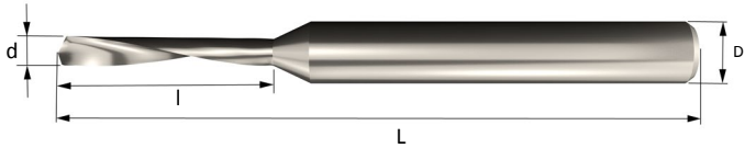
Style A | Carbide 1-Flute Twist Drill with Reinforced Shank
