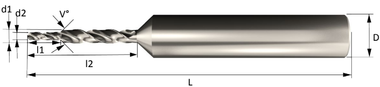
Style E | Carbide 2-Flute multiple Step Twist Drill with Reinforced Shank
