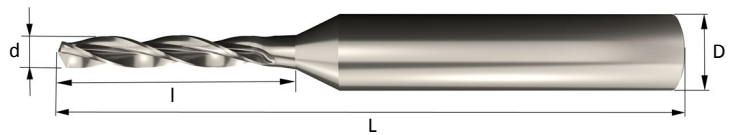
Style C | Carbide 3-Flute Twist Drill with Reinforced Shank
