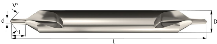
Style K | Carbide Double Countersink Drills
